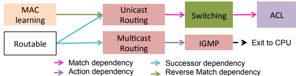
Figure 4: Table dependency graph for the L2L3 program.
