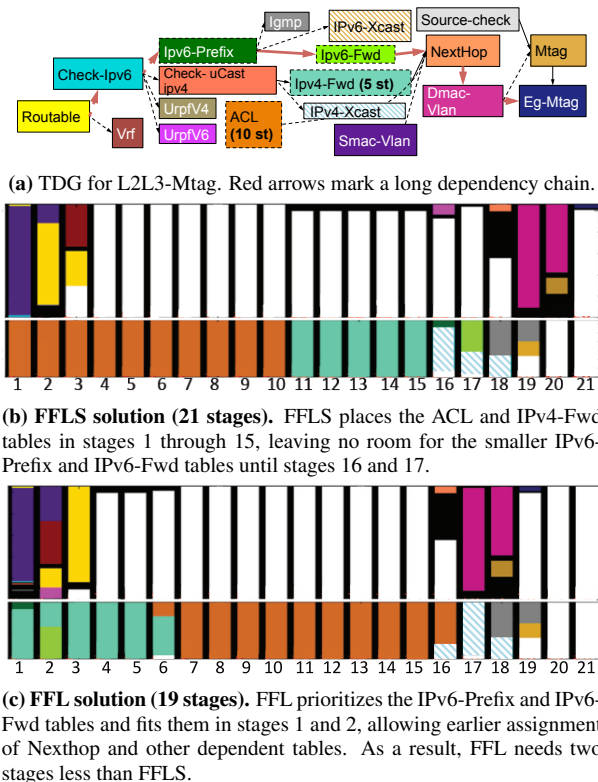
Figure 13: FFLS and FFL solutions for L2L3-Mtag. FFL prioritizes dependencies over table sizes and uses two fewer stages than FFLS.
