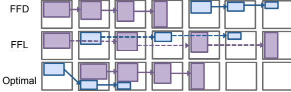
Figure 10: Greedy performing much worse than ILP (RMT). In this toy example, the blue and purple tables form separate match dependency chains. The initial blue table in the optimal mapping is narrower and has a lower level than the purple table, counterintuitive to both FFD and FFL metrics.
