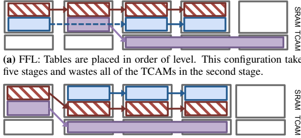
(b) FFLS: The first purple table with a large ternary table following it is placed first, even though the blue table has more match dependencies following it. This configuration uses only four stages.
